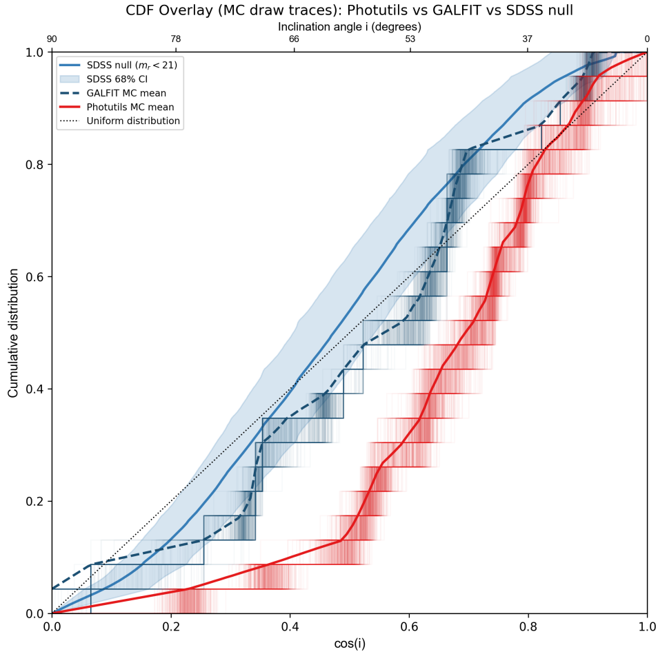
Figure 1: GALFIT and Photutils inclination comparisons against SDSS, including Monte Carlo uncertainty tracks.
