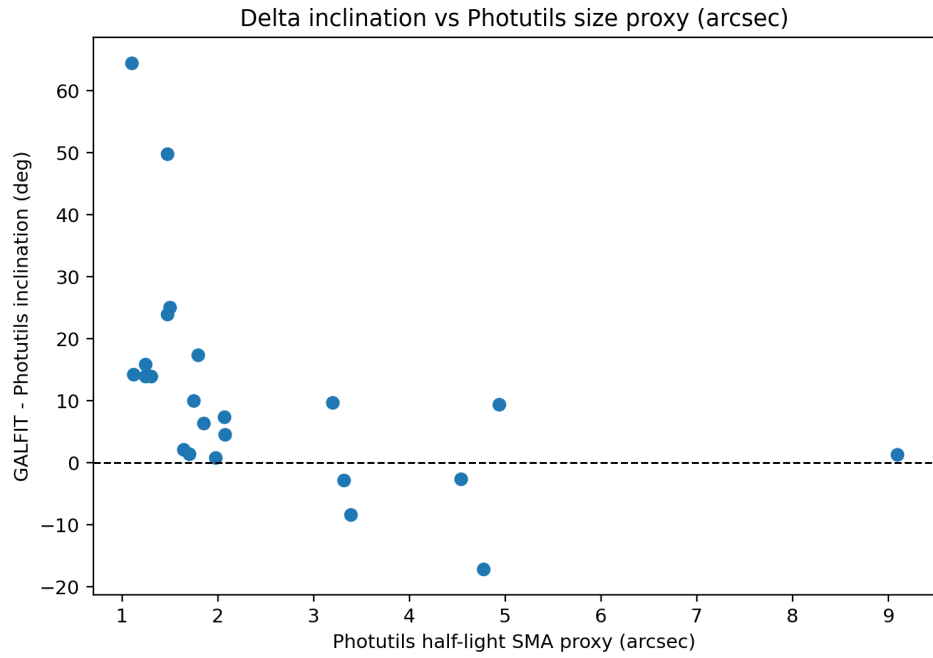
Figure 3: Difference in inclination (GALFIT - Photutils) vs. Photutils semi-major axis proxy in arcseconds.
