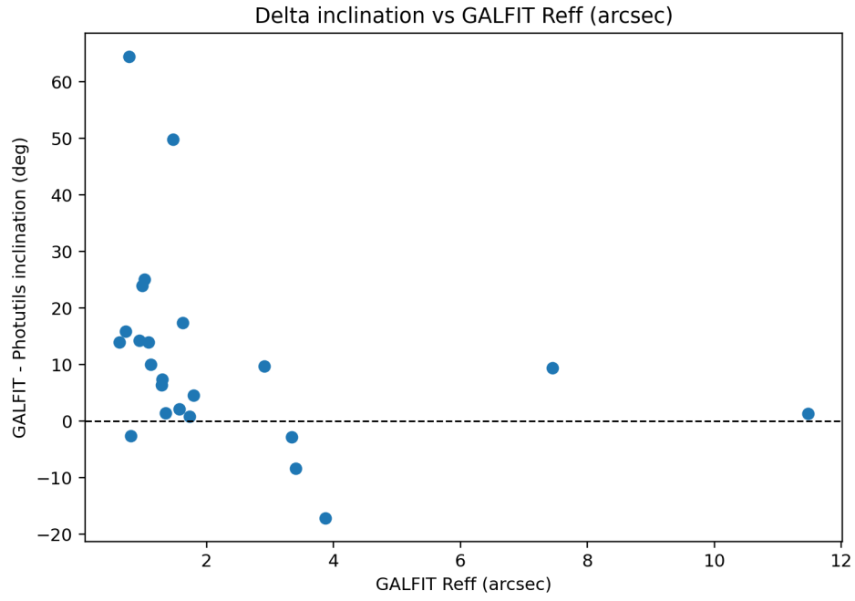
Figure 2: Difference in inclination (GALFIT - Photutils) vs. GALFIT effective radius in arcseconds.
