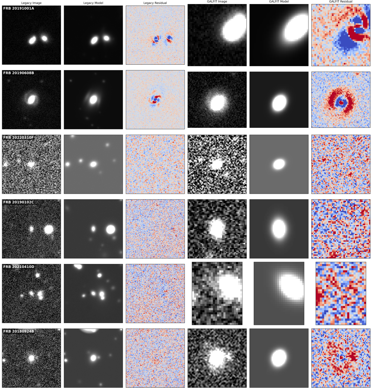
Figure 4: Top 6 inclination deviations (excluding REX), with FRB names labeled above each IMR row.
